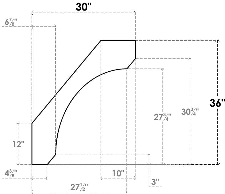
SIDE PROFILE
